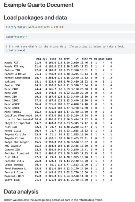
Figure 8.2: Preview of HTML file created from a Quarto file.
