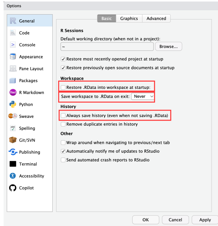
Figure 3.13: General options tab.
