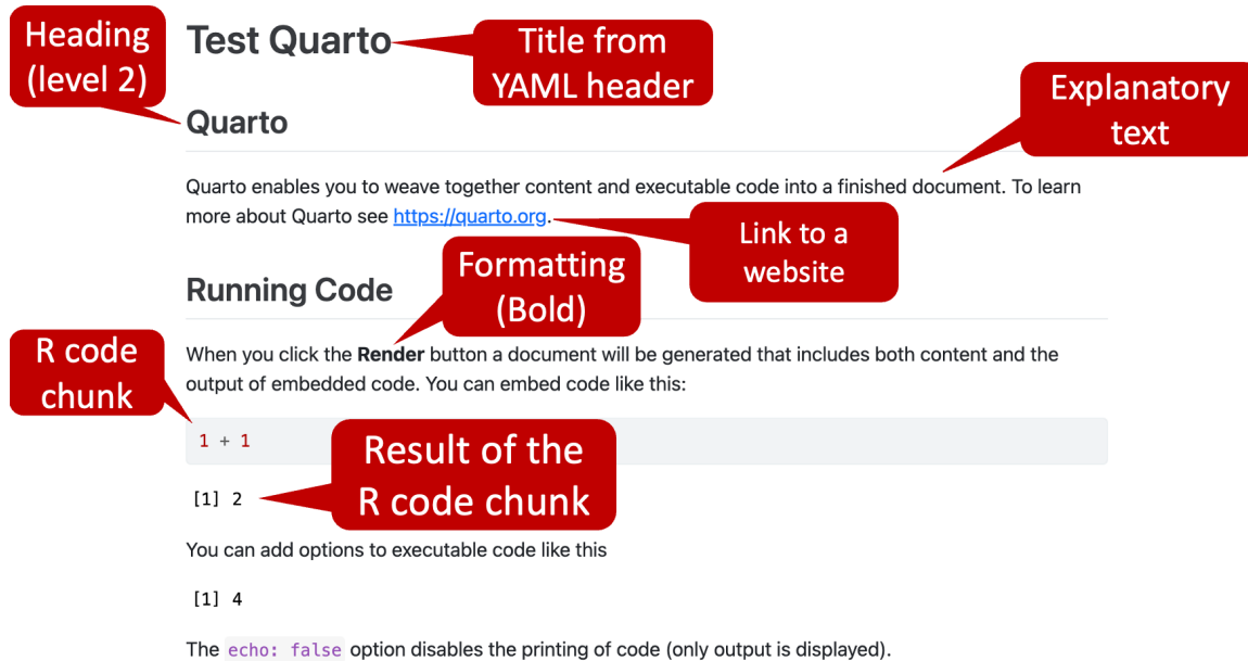
Figure 8.9: An HTML file created using a Quarto file.
