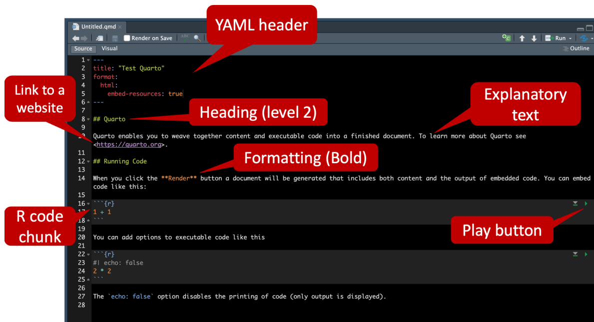
Figure 8.7: The ‘Test Quarto’ file in the RStudio source pane.
